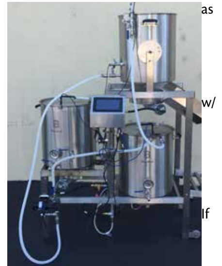
Hoses set up for Mash Recirculation
