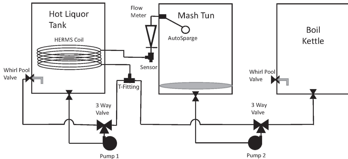
Plumbing and Hardware Schematic: 3 Vessel, Electric HERMS
