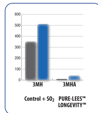
Figure 3: Sauvignon blanc wine trial comparing SO 2 addition (60 ppm) vs PURE-LEES LONGEVITY™ (40 g/hL): Thiols evaluation after 5 months of aging.
